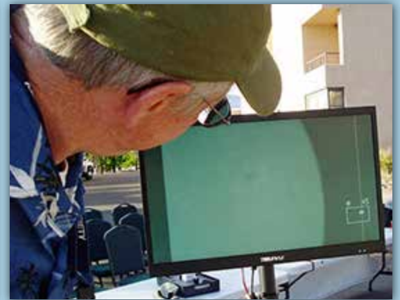
Live images of the Sun, and later deep sky objects, were projected from the telescope onto the monitor for the residents of La Vida Llena
