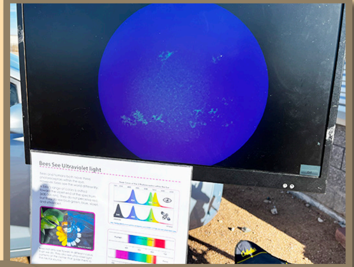
Live image of our Sun using a UV/calcium filter
