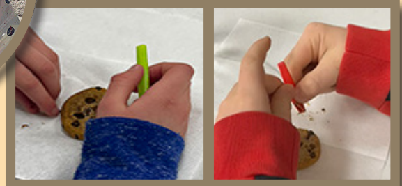
Spectroscopy on Mars--using a straw as a RAT (rock abrasion tool) campers took a core sample of the cookie--just like the Rover
